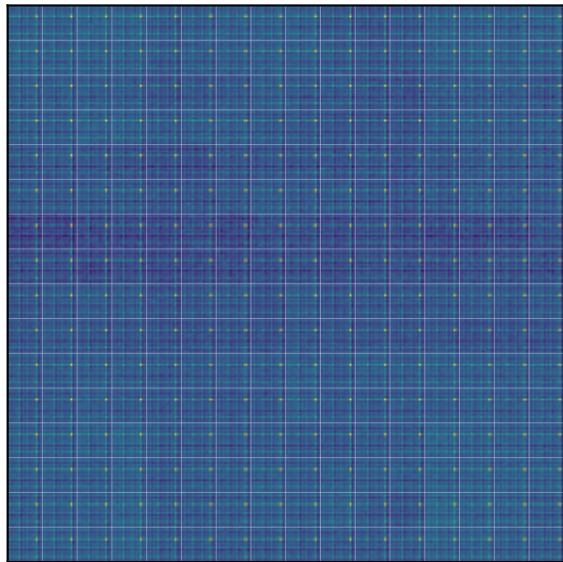
trained QFT (bg seed 28)
