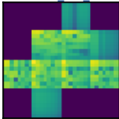
block_dct_8
