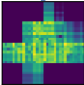
real_rich
