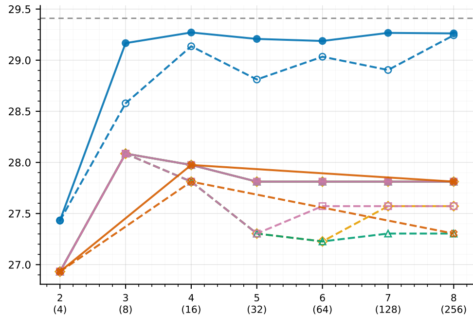
\rho = 0.1 (10 \times compression) · block-DCT-8 29.4 dB
