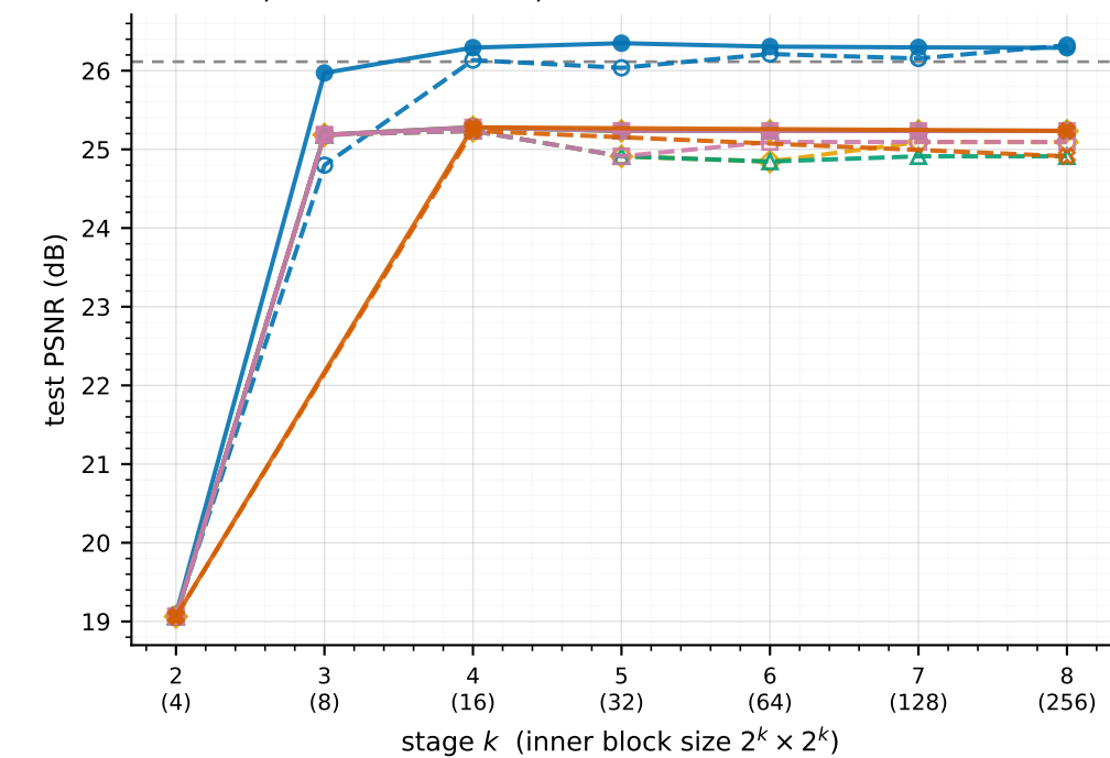
\rho = 0.05 (20 \times compression) · block-DCT-8 26.1 dB
