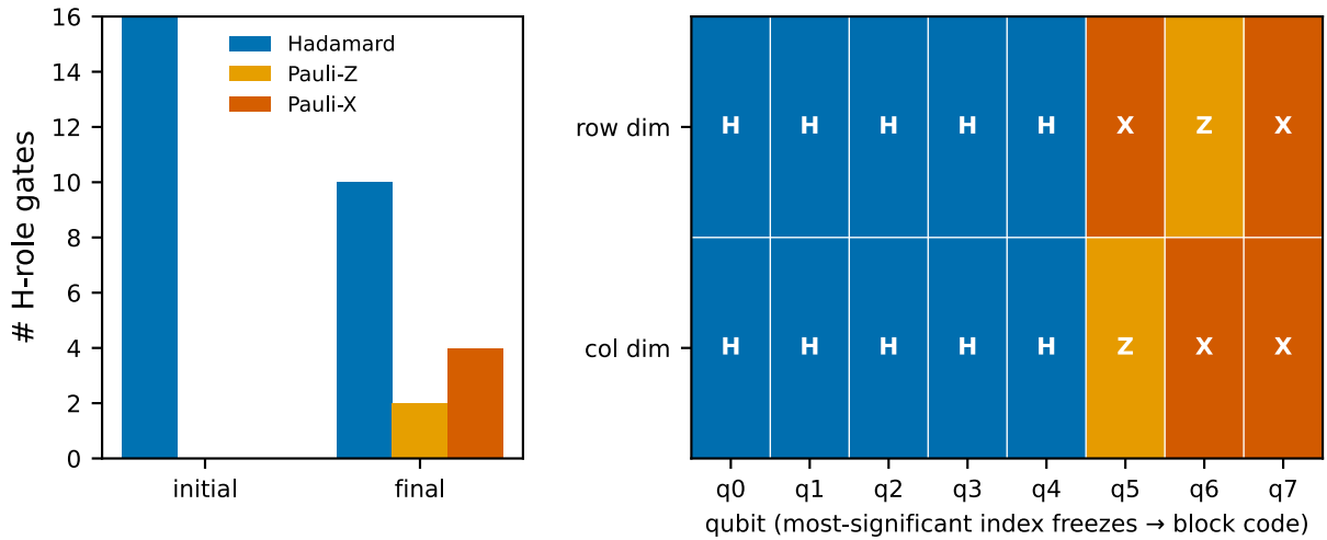
Figure 3: Left: H-role gate classification, initial vs final — all 16 gates begin as Hadamards and 6 freeze (2 to Pauli-Z, 4 to Pauli-X). Right: the exact locations — the most-significant qubits (q5– q7) collapse to Pauli (the classical block index) in both row and column dimensions, while q0– q4 stay Hadamard (the intra-block transform).
