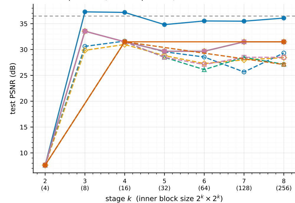
\rho = 0.05 (20 \times compression) · block-DCT-8 36.5 dB
