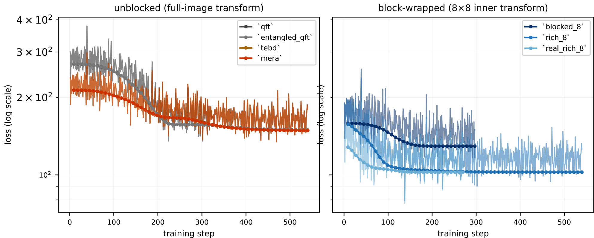
Figure 2: Per-step training loss (faint) and per-epoch validation loss (markers) for each trained basis on DIV2K-8q. Left panel: unblocked / full-image bases. Right panel: 8 \times 8 block-wrapped bases. Y-axis log-scale; identical scale across panels. Variable training lengths reflect early stopping at the validation-loss plateau. tebd and mera are visually indistinguishable here (the same curve to \geq 3 decimals across all training steps), consistent with their identical PSNR in the results table.
