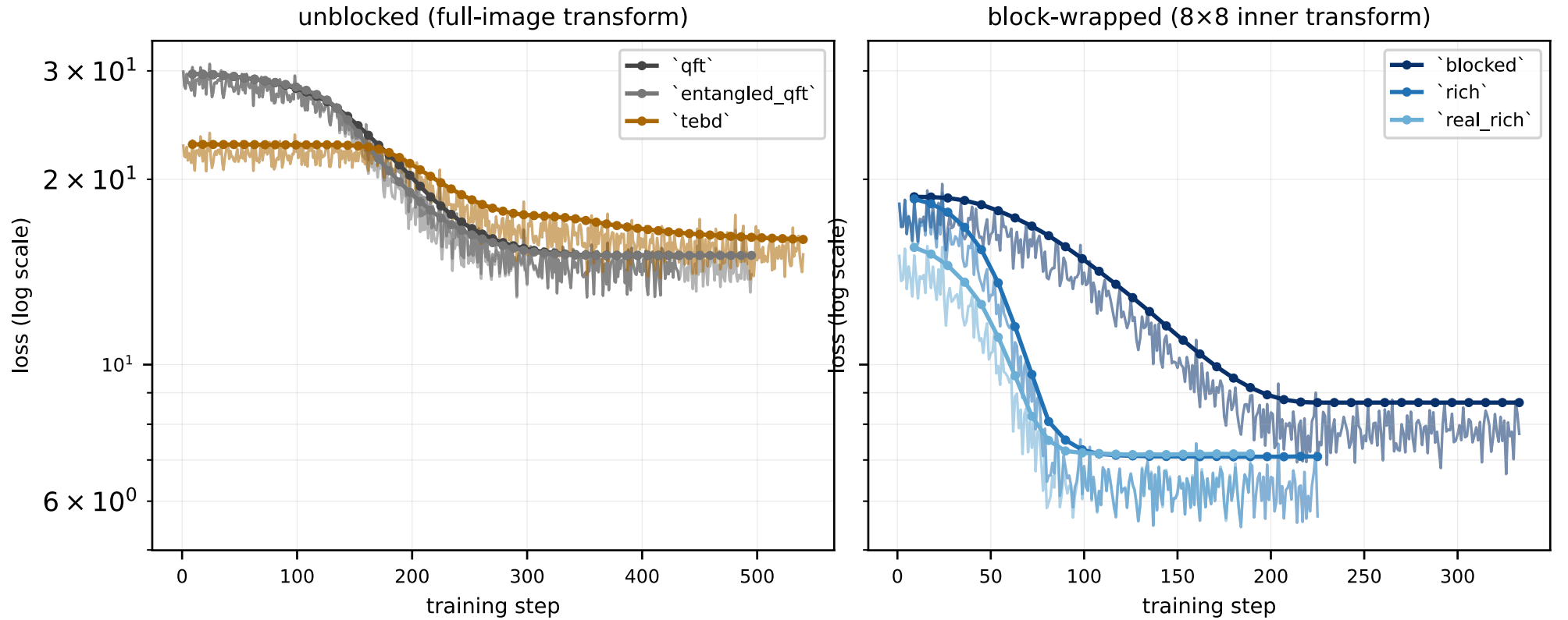
Figure 2: Per-step training loss (faint) and per-epoch validation loss (markers) for each trained basis on QuickDraw. Left panel: unblocked / full-image bases. Right panel: 8 \times 8 block-wrapped bases. Y-axis log-scale; identical scale across panels. Variable training lengths reflect early stopping at the validation-loss plateau. mera is omitted because m + n = 10 is not a power of 2 and the MERA hierarchy is structurally inapplicable.
