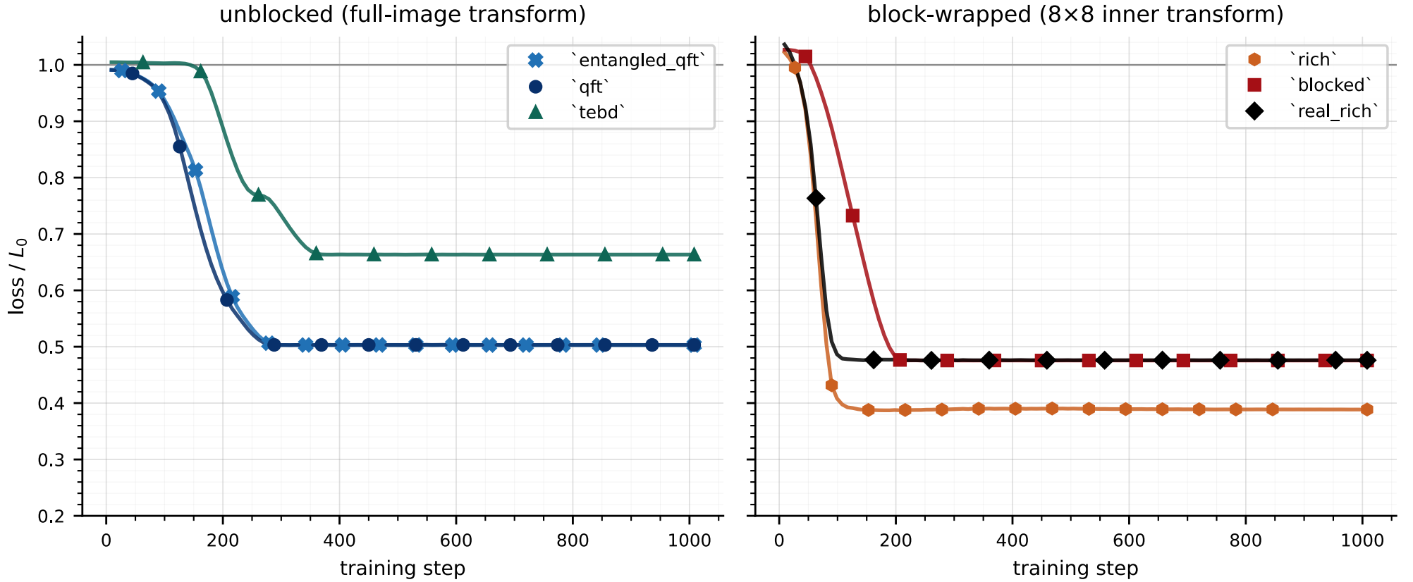
Figure 2: Per-epoch validation loss for each trained basis on QuickDraw at the headline 1008-step training budget. Y-axis is normalised by each basis’s own initial step-loss ( L/L_0 ); cross-basis comparison is on convergence speed and floor. Left: unblocked / full-image bases. Right: 8 \times 8 block-wrapped bases. Each basis is a (colour, marker, filled/hollow) triple from a colourblind-safe palette so every validation-checkpoint is observable as a discrete marker, no per-step noise overlay. mera is omitted because m + n = 10 is not a power of 2 and the MERA hierarchy is structurally inapplicable.
