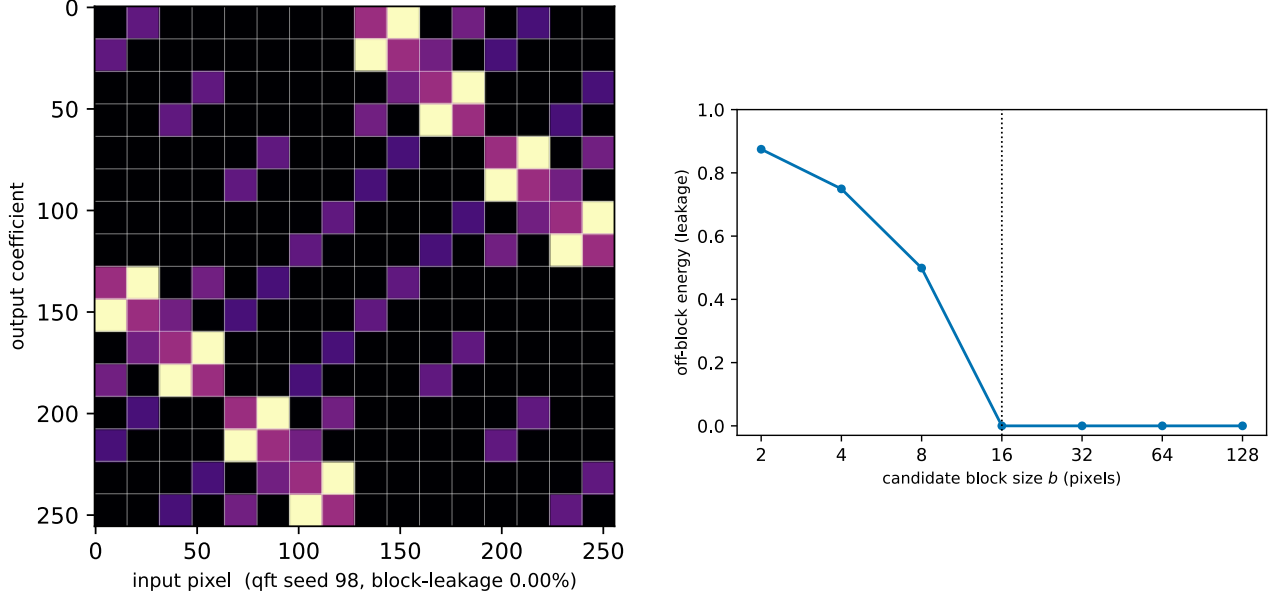
Figure 5: Left: \log|W| of the trained QFT’s 1-D operator factor, block-diagonal at the emergent 16-pixel block (off-block energy below 0.01%). Right: off-block energy vs candidate block size — the knee at b = 16 (dotted) shows the operator is block-structured at that specific scale and not below; the untrained closed-form QFT (not shown) stays high at every scale.
