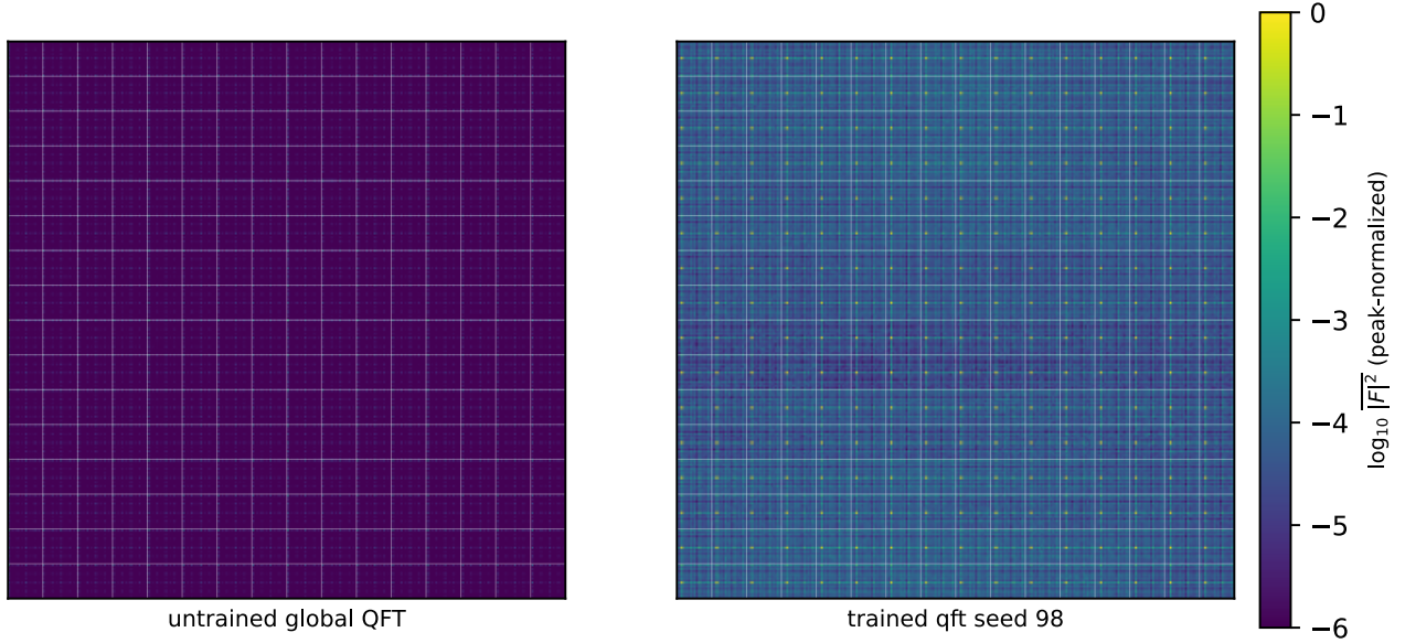
Figure 6: Mean test-set power spectrum (peak-normalized \log_{10} |F|^2 , averaged over the 50 DIV2K test images) of the untrained global QFT (left) and the trained QFT (right). The global transform packs energy into a single low-frequency lobe; the trained transform tiles into a 16 \times 16 grid of repeated sub-spectra — the block-periodic signature of a block transform, the same structure the 8 \times 8 block references produce in Fig. 4 of the main text.
