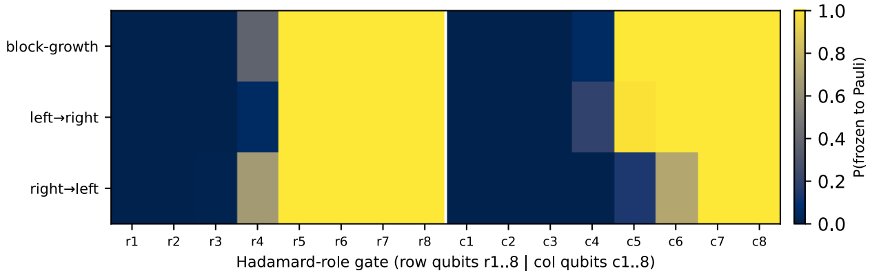
Figure 4: Per-Hadamard freeze probability across all seeds, one row per unfreeze ordering (row qubits r1..8 | col qubits c1..8). Roughly half of each dimension’s Hadamards reliably freeze to Pauli-Z/X (non-mixing), the rest stay frequency-mixing.
