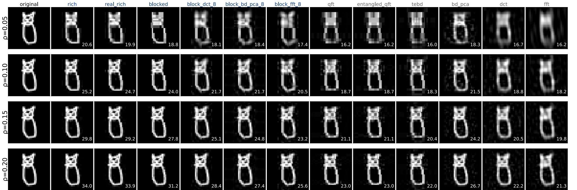
Figure 3: QuickDraw test image 0 reconstructed at four keep ratios \rho \in \{0.05, 0.10, 0.15, 0.20\} (rows). Same column order as the freq-space figure above. PSNR (dB) annotated bottom-right of each cell. At \rho = 0.20 : trained rich \approx 34 dB vs block_dct_8 \approx 28 dB (+6 dB) vs dct \approx 22 dB (+12 dB).
