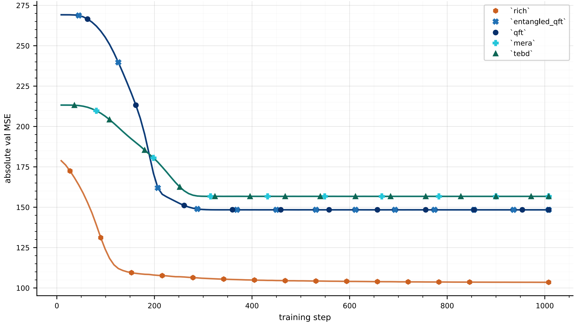
Figure 2: Per-epoch validation MSE for the five learned full-image bases (RichBasis, qft , entangled_qft , mera , tebd ) on DIV2K-8q at the headline 1008-step training budget (canonical init, seed 42, \rho = 0.10 training objective). All share a single linear y-axis: absolute MSE, the operational quantity (max PSNR \equiv min MSE), so the right-edge curve ordering reproduces the headline PSNR ranking by inspection — rich (RichBasis) reaches the lowest floor ( \approx 103 ), the qft / entangled_qft pair sits at \approx 148 , and the tebd / mera pair at \approx 157 . Each basis is a (colour, marker) pair from a colourblind-safe palette; the coincident pairs ( qft \equiv entangled_qft , tebd \equiv mera ) overlap exactly because their parametric families compile to the same operator at this circuit depth. Loss is essentially flat past step \approx 300 for every basis (the appendix plateau check at 2000 steps moves headline values by \leq 0.01 dB).
