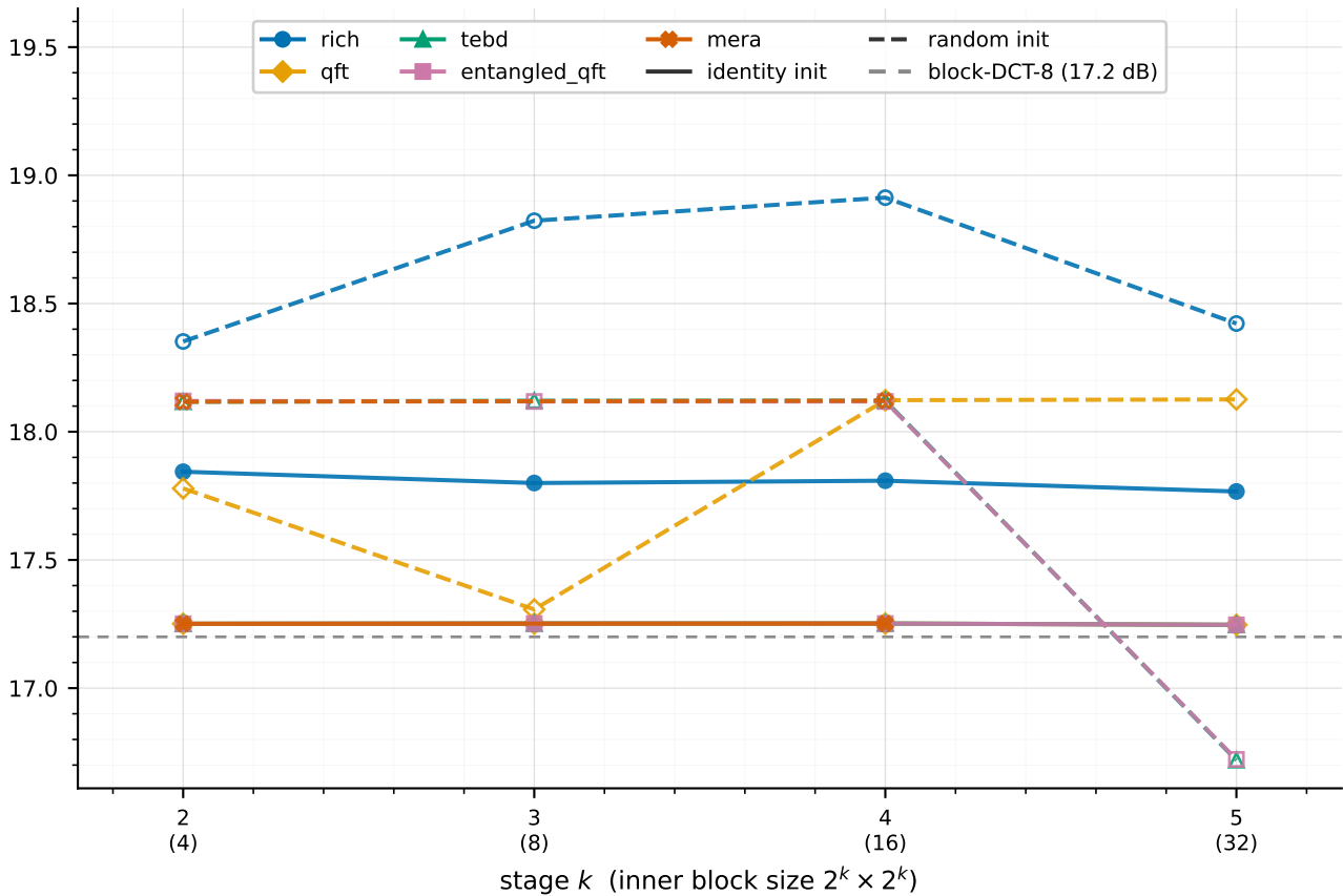
test PSNR @ \rho = 0.05 (20x compression) (dB)
