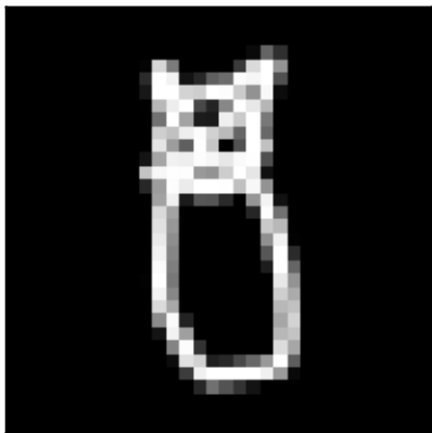
L1 ( \lambda=10 )
