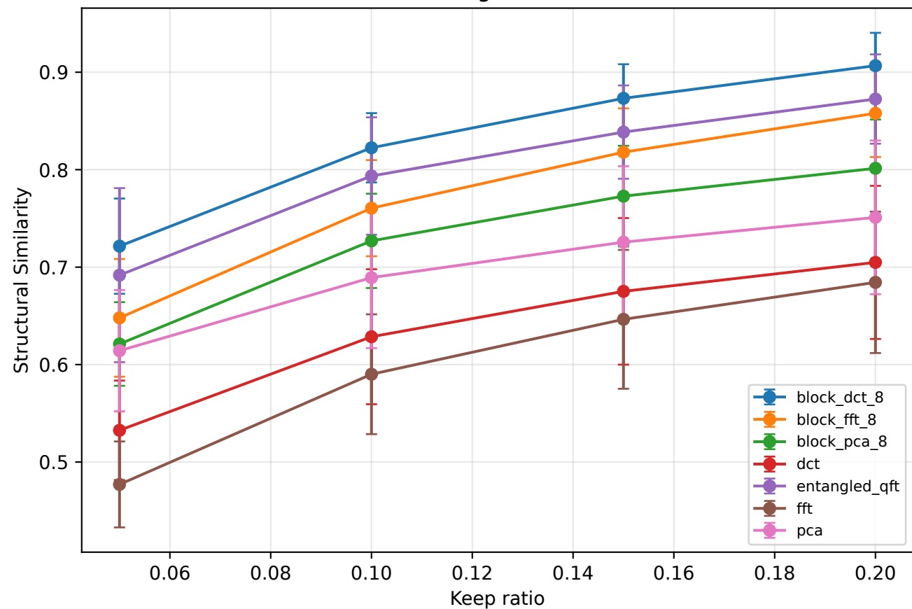
SSIM — higher is better
