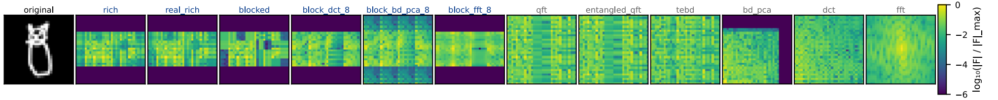
Figure 3: Frequency-space spectra (peak-normalised \log|F| , viridis, shared color scale) for image 0 under each basis. Same column order as the recon grid below. Note the trained block-wrapped bases (blue headers) push energy into a small number of low-coefficient cells per block — visible as the bright clusters in rich/real_rich/blocked and the band structure in block_dct_8/block_bd_pca_8. The bd_pca panel shows energy concentrated in the top-left corner (low-frequency / high-eigenvalue) along both axes — the separable-KLT analog of the DCT spectrum.
