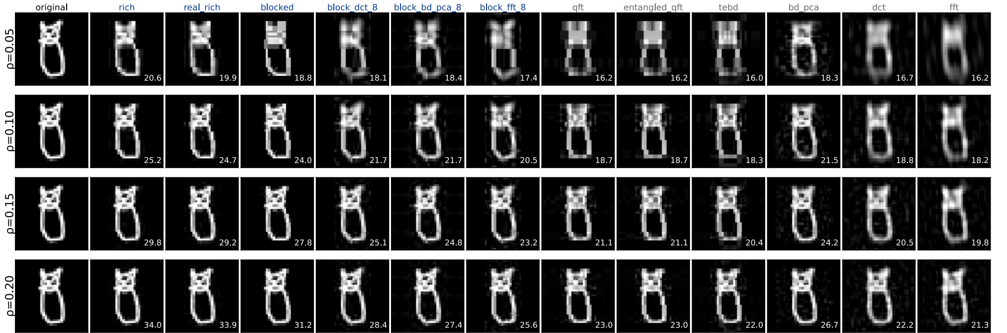
Figure 4: QuickDraw test image 0 reconstructed at four keep ratios \rho \in \{0.05, 0.10, 0.15, 0.20\} (rows). Same column order as the freq-space figure above. PSNR (dB) annotated bottom-right of each cell. At \rho = 0.20 : trained rich \approx 34 dB vs block_dct_8 \approx 28 dB (+6 dB) vs dct \approx 22 dB (+12 dB).
