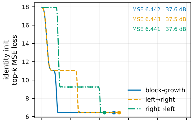
QuickDraw (m=n=5)
