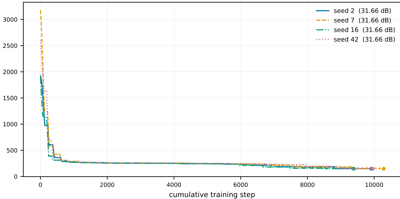
training top-k MSE loss
