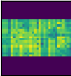
rich
