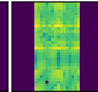
block DFT 8x8
