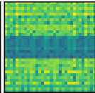
Entangled QFT
