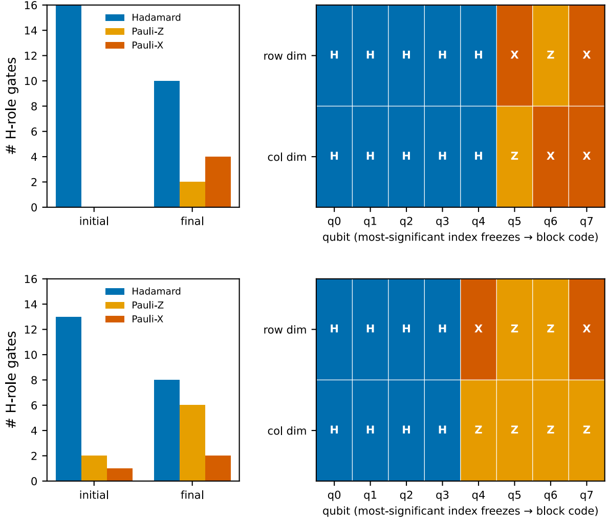
Figure 3: Gate freezing for two initialisations. Top: seed 0 — 6 gates freeze (q5–q7 per dimension) into the 32-px block. Bottom: seed 98, the canonical paper operator — 8 freeze (q4–q7) into the finer 16-px block. Left panels: H / Pauli-Z / Pauli-X counts, initial vs final; right panels: the exact frozen qubit positions. The most-significant qubits always collapse to Pauli; the initialisation sets how many.
