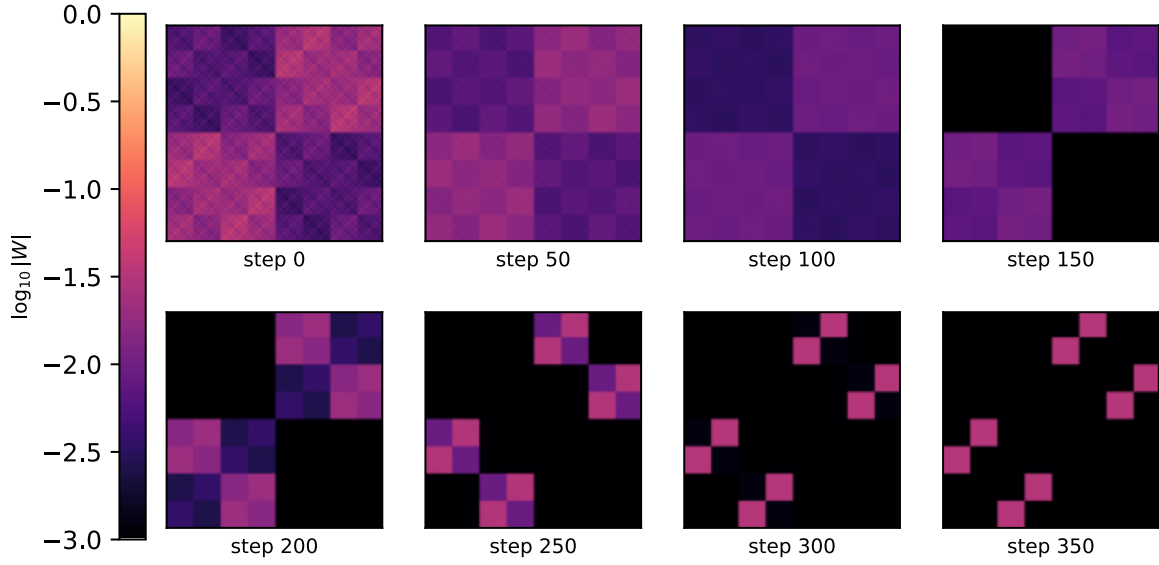
Figure 2: The operator’s 1-D factor \log_{10}|W| at eight training steps. The Haar init (step 0) is dense — every input pixel drives every output coefficient. As gates freeze, |W| collapses onto a block-diagonal (up to the QFT bit-reversal + frozen-X permutation), ending at 8 blocks of 32 pixels. This is the operator-space twin of the frequency-space spectrogram above: the off-block energy draining away is the comb sharpening.
