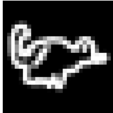
QuickDraw #2 \hat{\rho}=0.71
