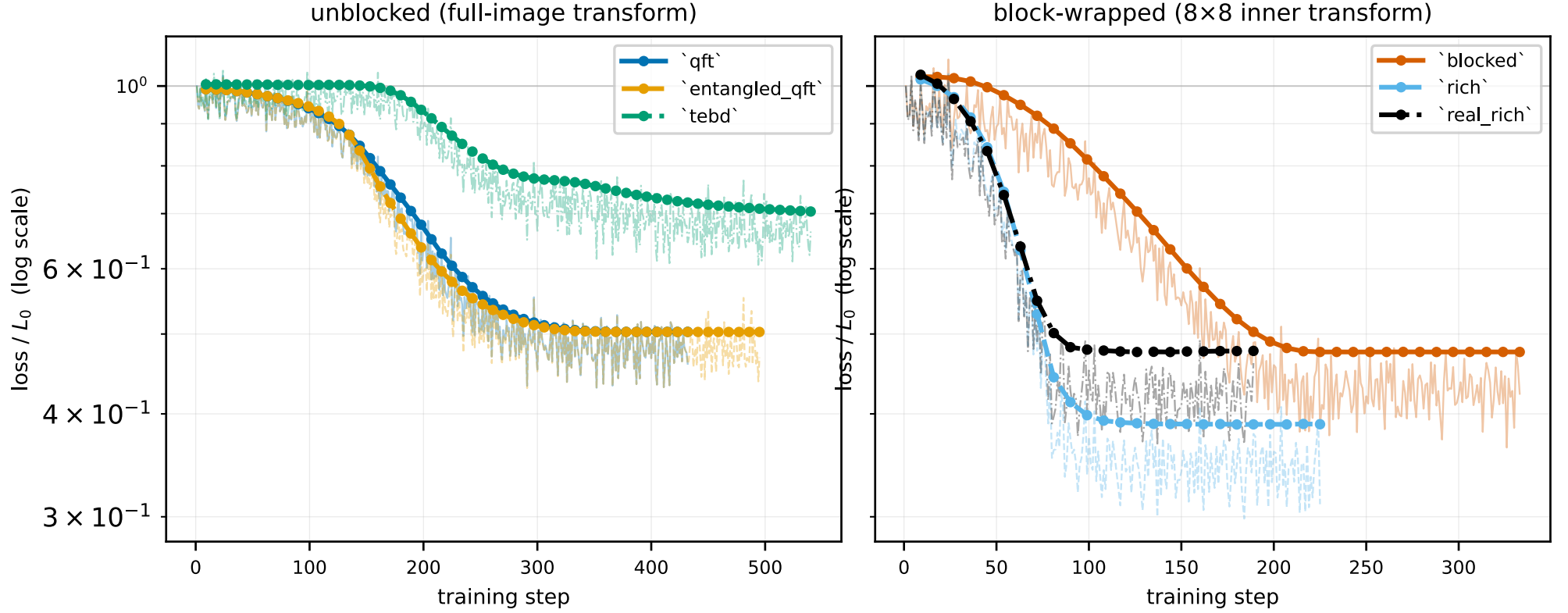
Figure 2: Per-step training loss (faint) and per-epoch validation loss (markers) for each trained basis on QuickDraw. Y-axis is normalised by each basis's own initial step-loss ( L/L_0 , log scale) so every curve starts at 1.0 and cross-basis comparison is on convergence speed and floor rather than raw scale. Left panel: unblocked / full-image bases. Right panel: 8 \times 8 block-wrapped bases. Each basis uses a unique colour + line-style pair from a colourblind-safe palette. Variable training lengths reflect early-stopping at the validation-loss plateau. mera is omitted because m + n = 10 is not a power of 2 and the MERA hierarchy is structurally inapplicable.
