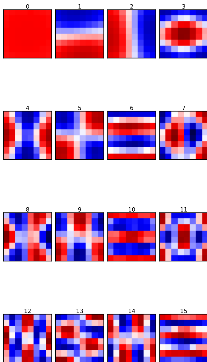
block_PCA — top-16 eigen-patches (8×8) rows of \Phi_b \in \mathbb{R}^{64 \times 64} , fit on 512000 patches
