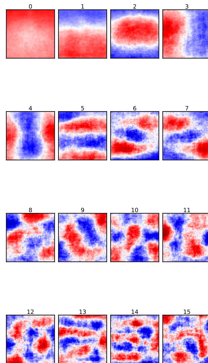
global PCA — top-16 eigen-images (256×256) rows of \Phi \in \mathbb{R}^{65536 \times 65536} , fit on 500 images
