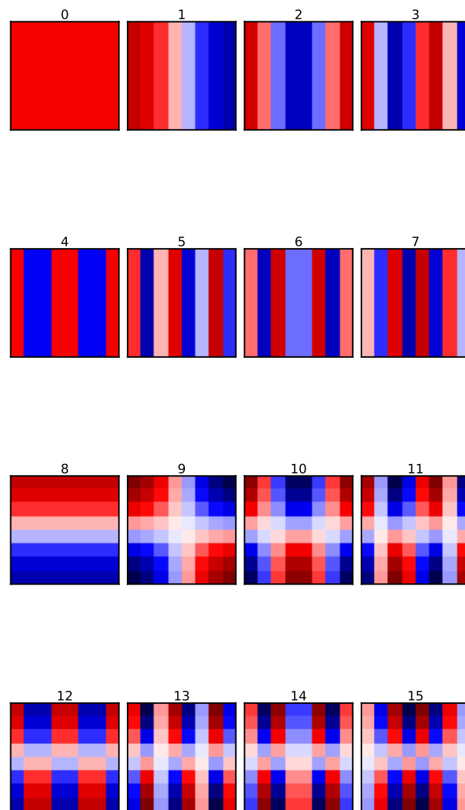
block_DCT (closed-form) — first 16 basis patches (8×8) \Phi[k, \cdot] = \cos(\pi(n + \frac{1}{2})k/8) — for reference
