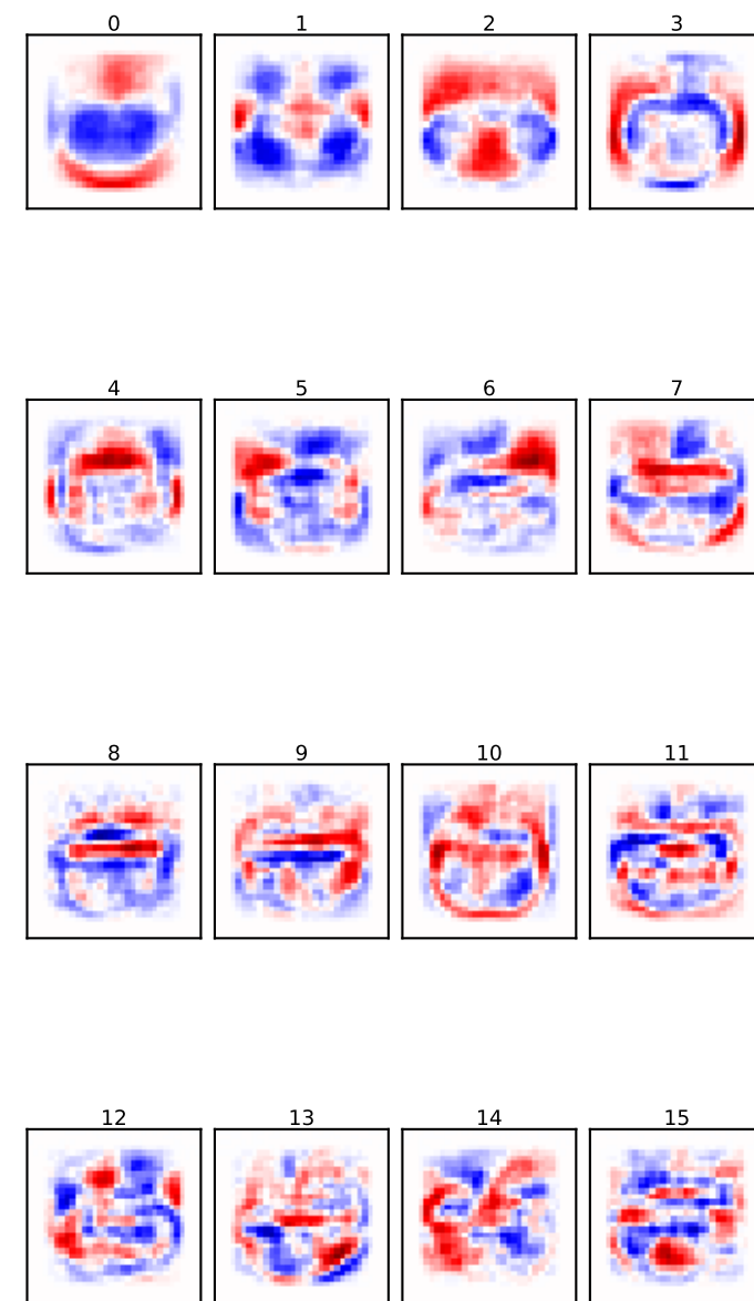
global PCA — top-16 eigen-images ( 32 \times 32 ) rows of \Phi \in \mathbb{R}^{\{1024 \times 1024\}} , fit on 500 images
