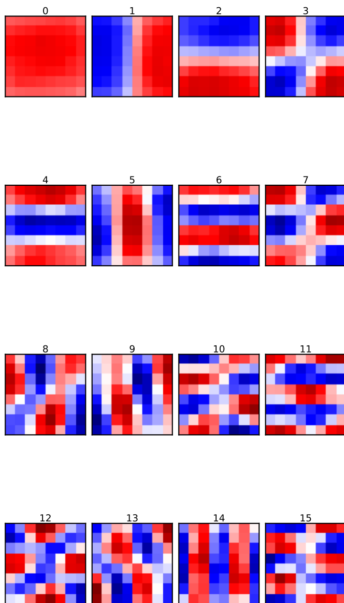
block_PCA — top-16 eigen-patches ( 8 \times 8 ) rows of \Phi_b \in \mathbb{R}^{\{64 \times 64\}} , fit on 8000 patches
