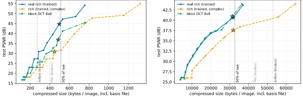
Figure 1: Rate-distortion in real bytes per image (blob + amortised basis file). Left: QuickDraw. Right: DIV2K-8q. Stars mark the best operating point within the 50%-of-raw budget (dotted vertical). Grey dotted verticals: lossless deflate / PNG references.
