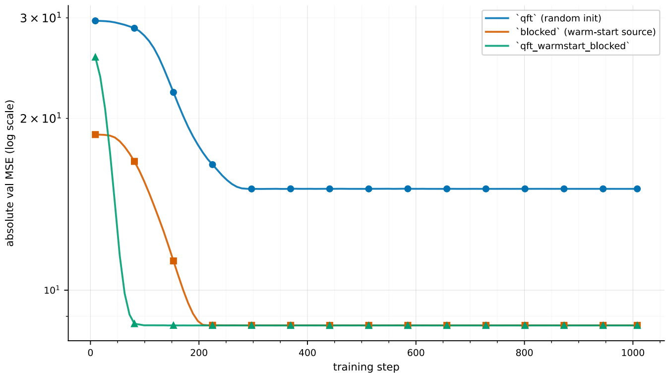
Figure 2: QuickDraw. Validation MSE per training step (log y). Blue: qft from random init. Orange: blocked headline run (warm-start source). Green: qft_warmstart_blocked . The warm-started run is bit-exact equal to the trained blocked operator at step 0; the cosine-LR warmup briefly perturbs it away from the blocked optimum before Adam pulls it back to the blocked floor by step \approx 200 and stays there. Loss definition: \sum_{ij} \left| x_{ij} - \left( T_{\theta}^{\dagger} \text{top}_K(T_{\theta} x) \right)_{ij} \right|^2 summed over 1024 pixels of a 32 \times 32 image at K = 102 ( \rho = 0.10 ), averaged over the 75-image validation split.
