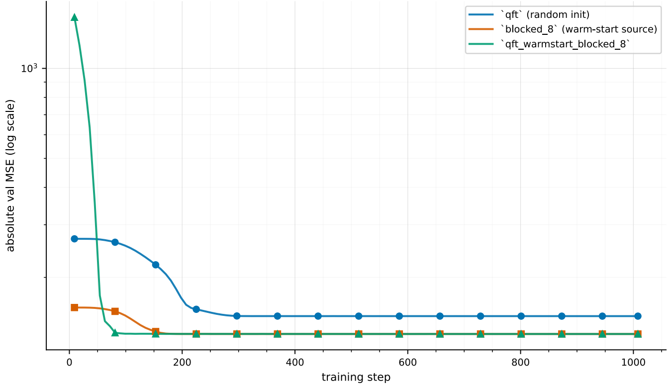
Figure 1: DIV2K-8q. Validation MSE per training step (log y). Blue: qft from random init. Orange: blocked_8 headline run (warm-start source). Green: qft_warmstart_blocked_8 . The log y compresses a real \approx 10 \times dynamic range — the cosine-LR warmup briefly throws the warm-started operator far above its starting MSE before Adam pulls it back to the blocked floor by step \approx 100 , where it stays for the remaining 900 steps. Loss definition: \sum_{ij} \left| x_{ij} - \left( T_{\theta}^{\dagger} \text{top}_K(T_{\theta} x) \right)_{ij} \right|^2 summed over 65536 pixels of a 256 \times 256 image at K = 6554 ( \rho = 0.10 ), averaged over the 75-image validation split.
