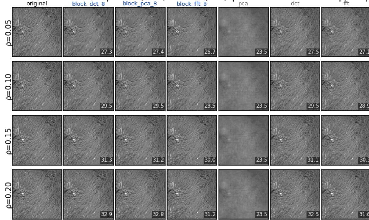
Figure 5: DIV2K-8q test image #43 (smoothest) reconstructed at the same four keep ratios. Same column layout as image #11. Smooth imagery is the easiest case for any sparsifying transform: at \rho = 0.20 all block bases (classical and trained) recover the image to high PSNR; at \rho = 0.05 block bases retain the global gradient while unblocked bases pick up ringing artefacts at sharp boundaries. pca is again pinned at 18.15 dB — the rank-499 ceiling limits even smooth-image reconstruction.
