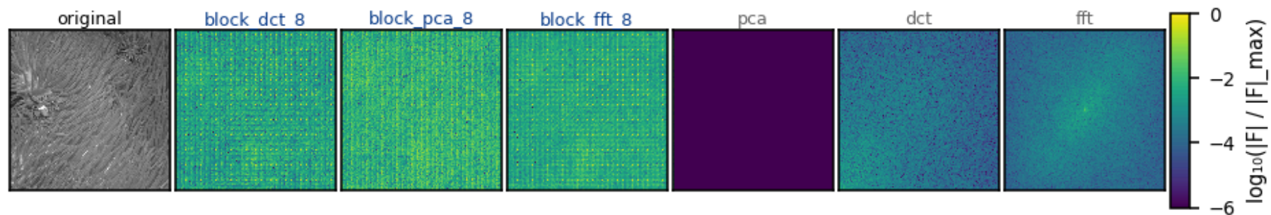
Figure 4: Frequency-space spectra for image #43 (smoothest test image, stdev \approx 0.08 ). Same column layout as the image-#11 freq panel. Smooth content concentrates almost all energy into the DC and low-frequency cells per block, so even small keep ratios capture most of the image — the block bases' freq panels are sparser than image #11's.
