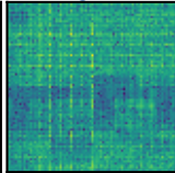
Entangled QFT
