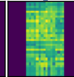
real_rich
