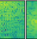
dct
