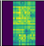
rich
