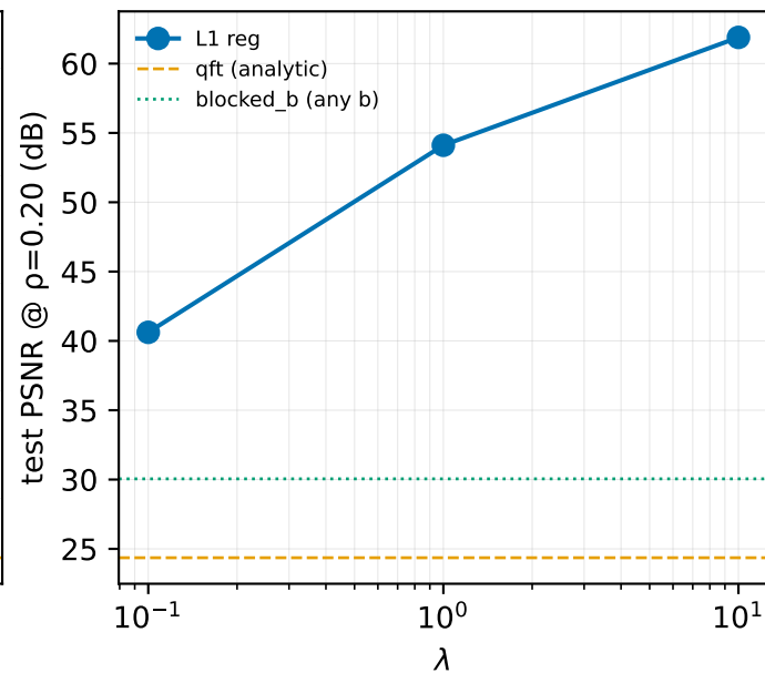
QuickDraw (m=n=5)
