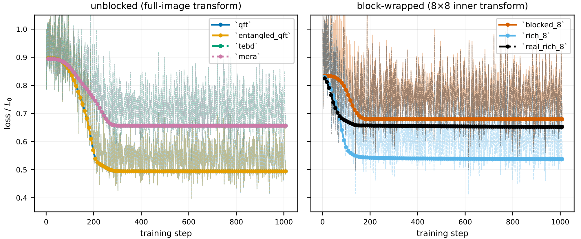
Figure 2: Per-step training loss (faint) and per-epoch validation loss (markers) for each trained basis on DIV2K-8q at the headline 1008-step training budget. Y-axis is normalised by each basis’s own initial step-loss ( L/L_0 ); cross-basis comparison is on convergence speed and floor. Left: unblocked / full-image bases. Right: 8 \times 8 block-wrapped bases. Each basis gets a unique colour + line-style pair from a colourblind-safe palette. The training-loss windowed average is essentially flat past step 700 for every basis (gain past step 1000 is \leq 0.01 dB equivalent — see appendix plateau check), justifying 1000 steps as the headline budget.
