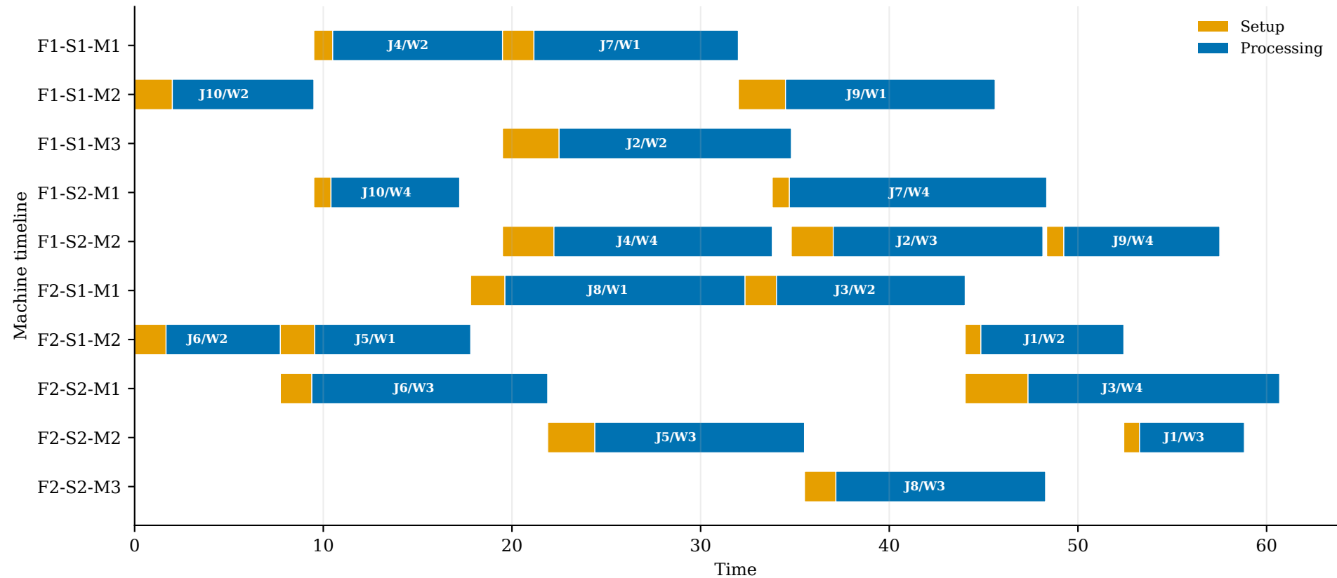
I1/X0 machine Gantt chart under FM0
