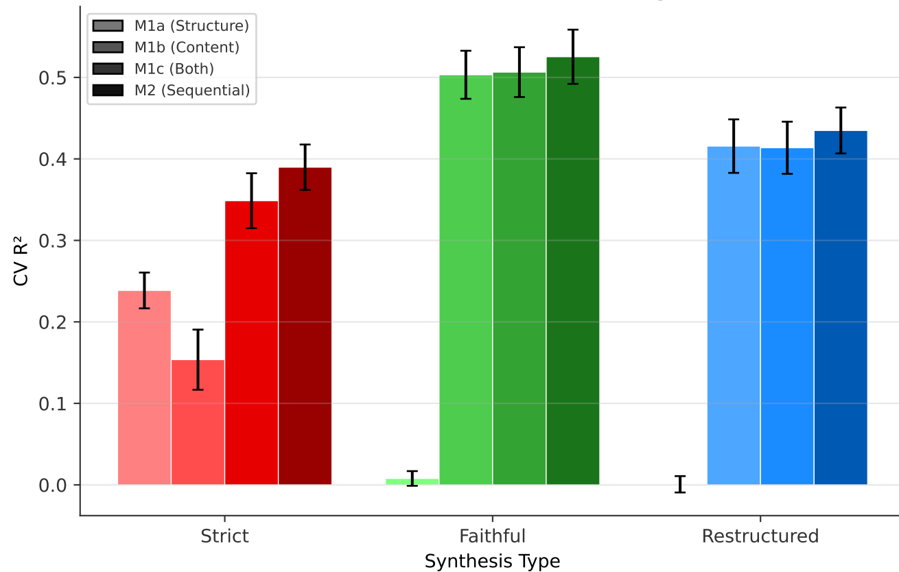
(A) Cross-Validation Performance (Intervals show observed range)
