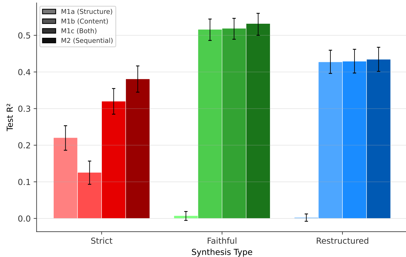
(B) Test Set Performance (95% CI)
