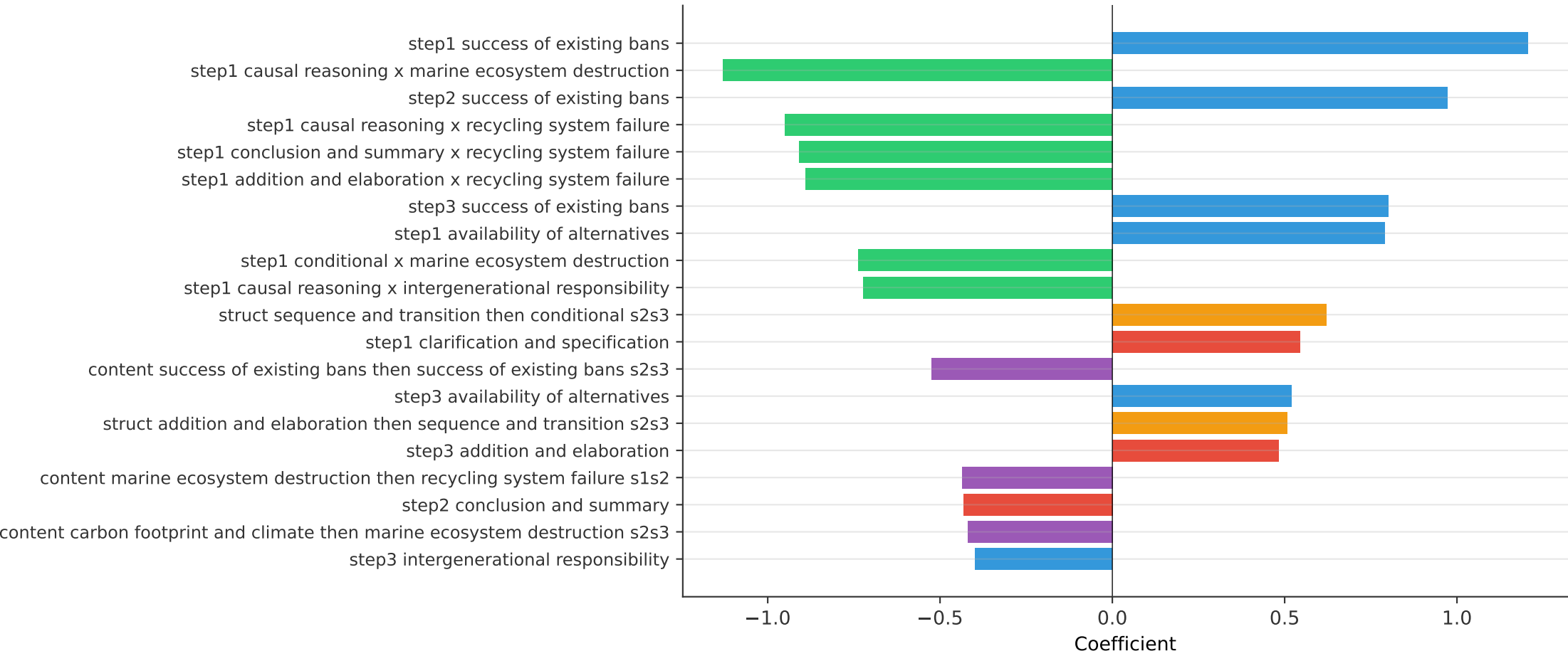
Faithful - Top 20 Features (|coef|)
