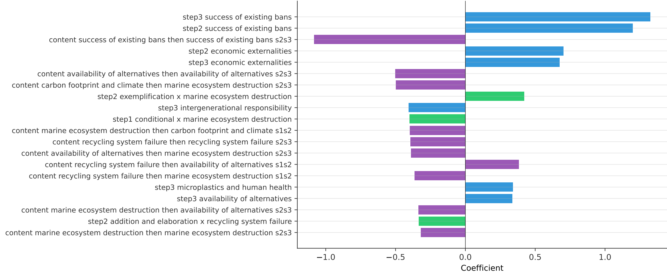
Restructured - Top 20 Features (|coef|)
