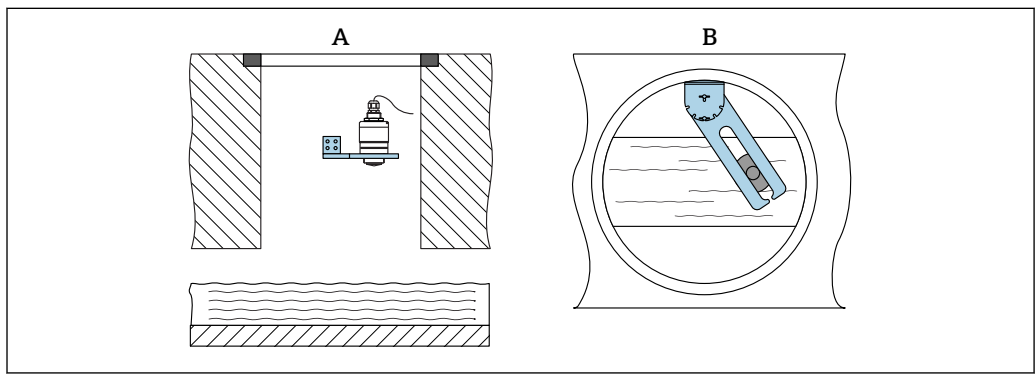
21 Mounting in a shaft, pivotable and adjustable
