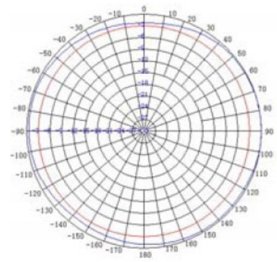
H Plane Pattern
