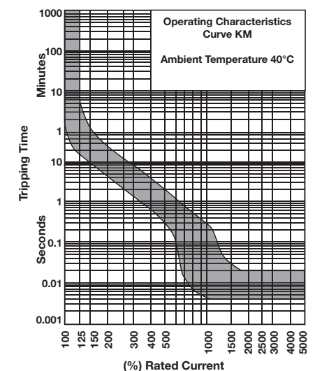
9926 Series-AC version
