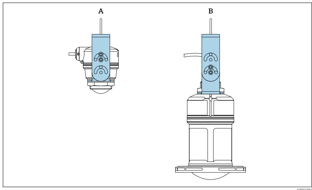
17 Installation with rope mounting
