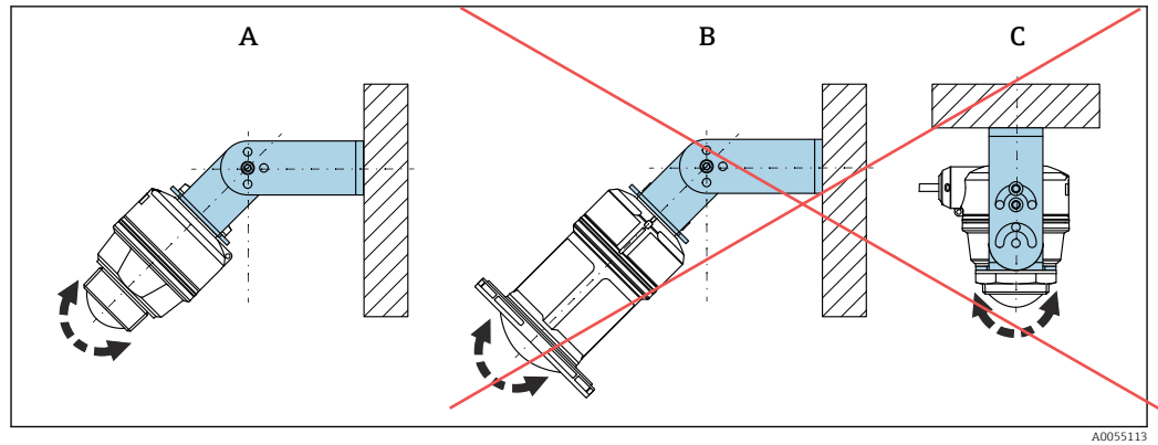
16 Installation with mounting bracket, adjustable
