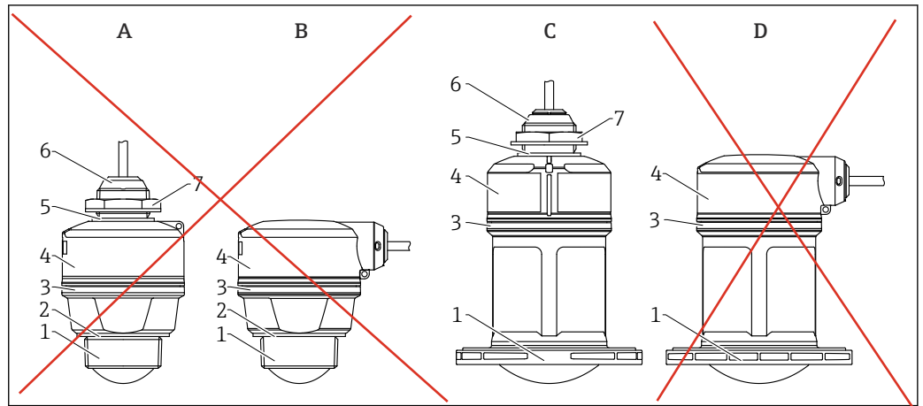
26 Device design
