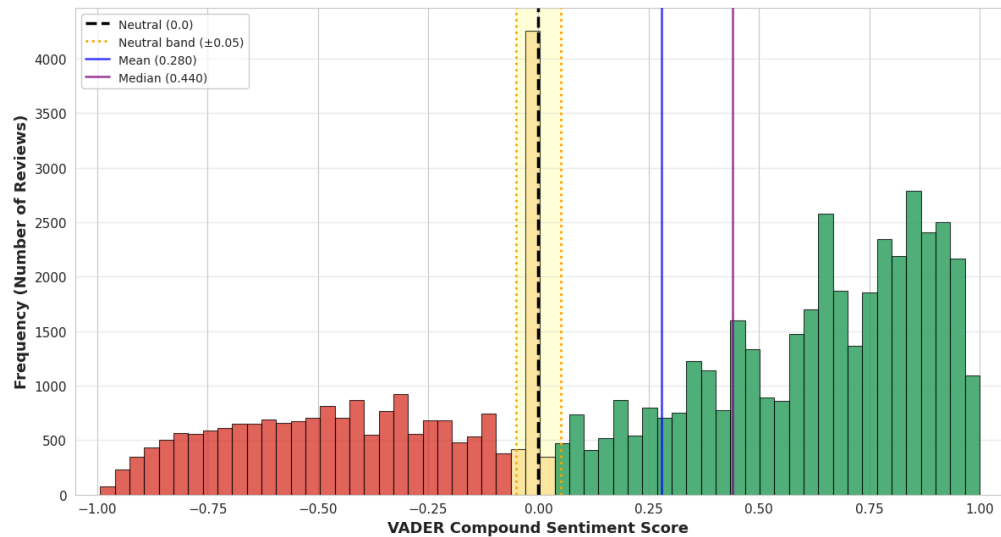
Figure 2: Distribution of VADER Compound Sentiment Scores
