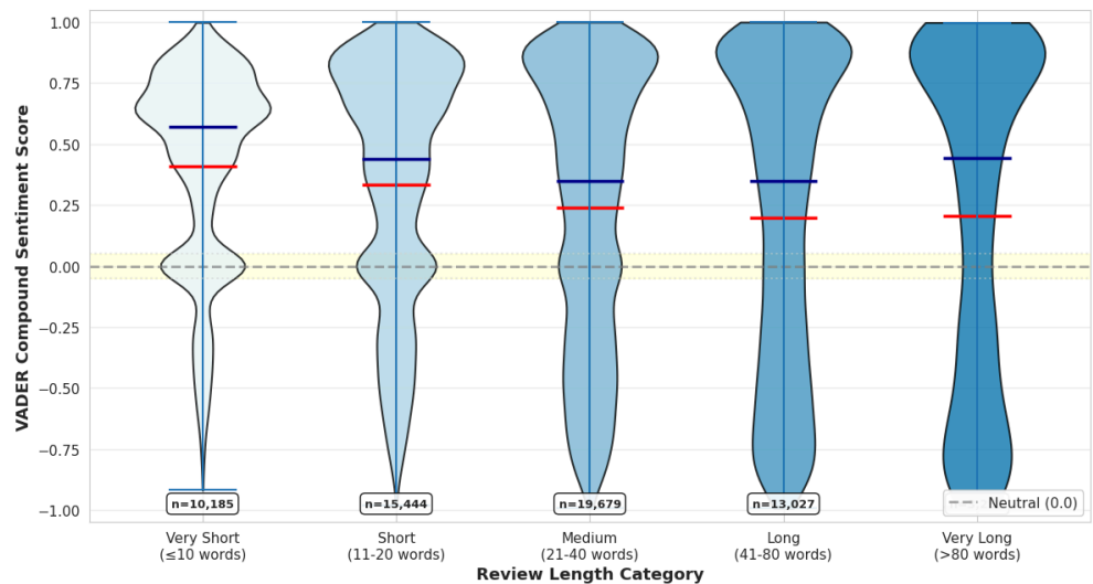
Figure 1: Sentiment Distribution Across Review Length Categories
