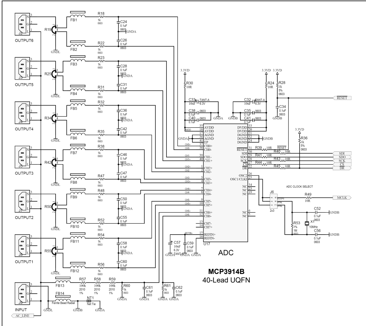
FIGURE 7-1: MCP3914B Power Strip Application Example Schematic (may be used as starting point for MCP3913B applications).
