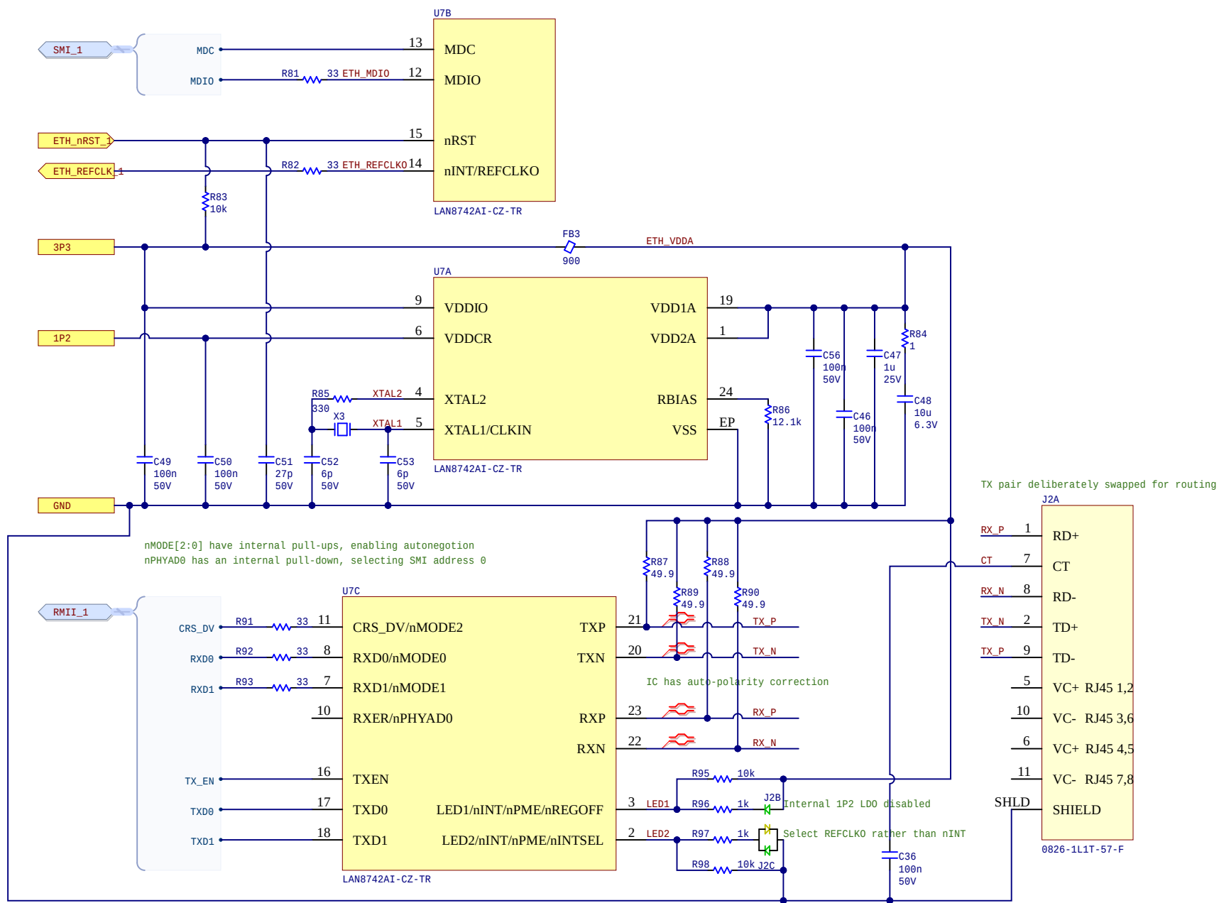
RMII-interface 100Base-TX PHY
