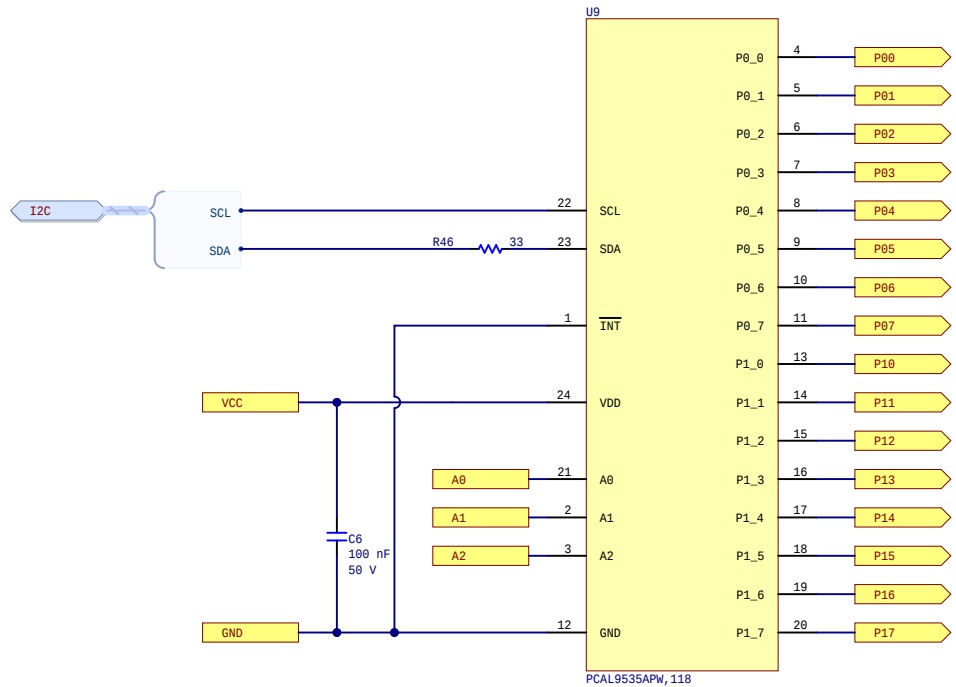
Bidirectional I2C GPIO expander
