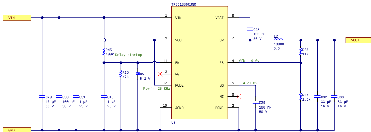
5 volt, 6 amp output buck converter
