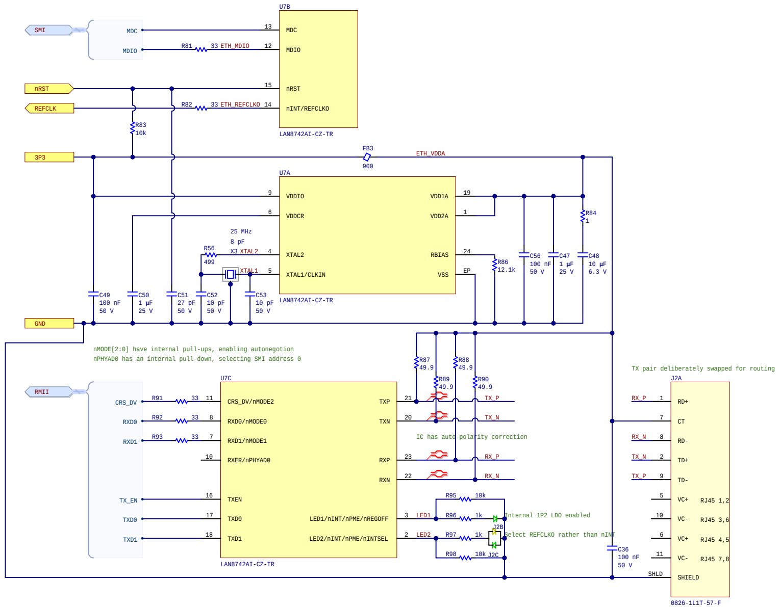
RMII-interface 100Base-TX PHY
