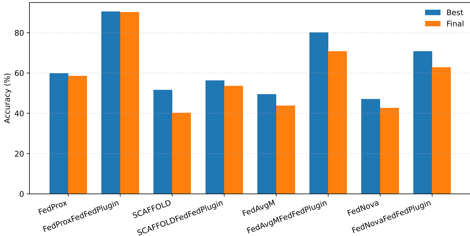
FedFed plugin across FL backbones
