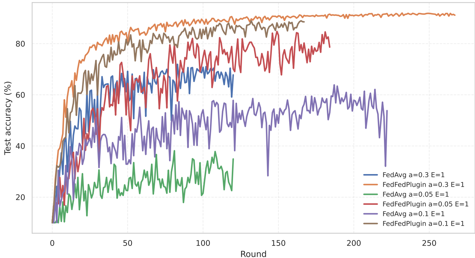
heterogeneity_alpha: accuracy curves
