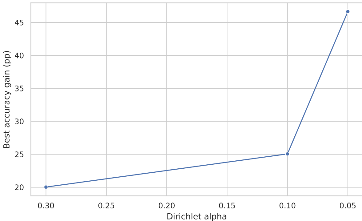
FedFed gain under label/quantity skew
