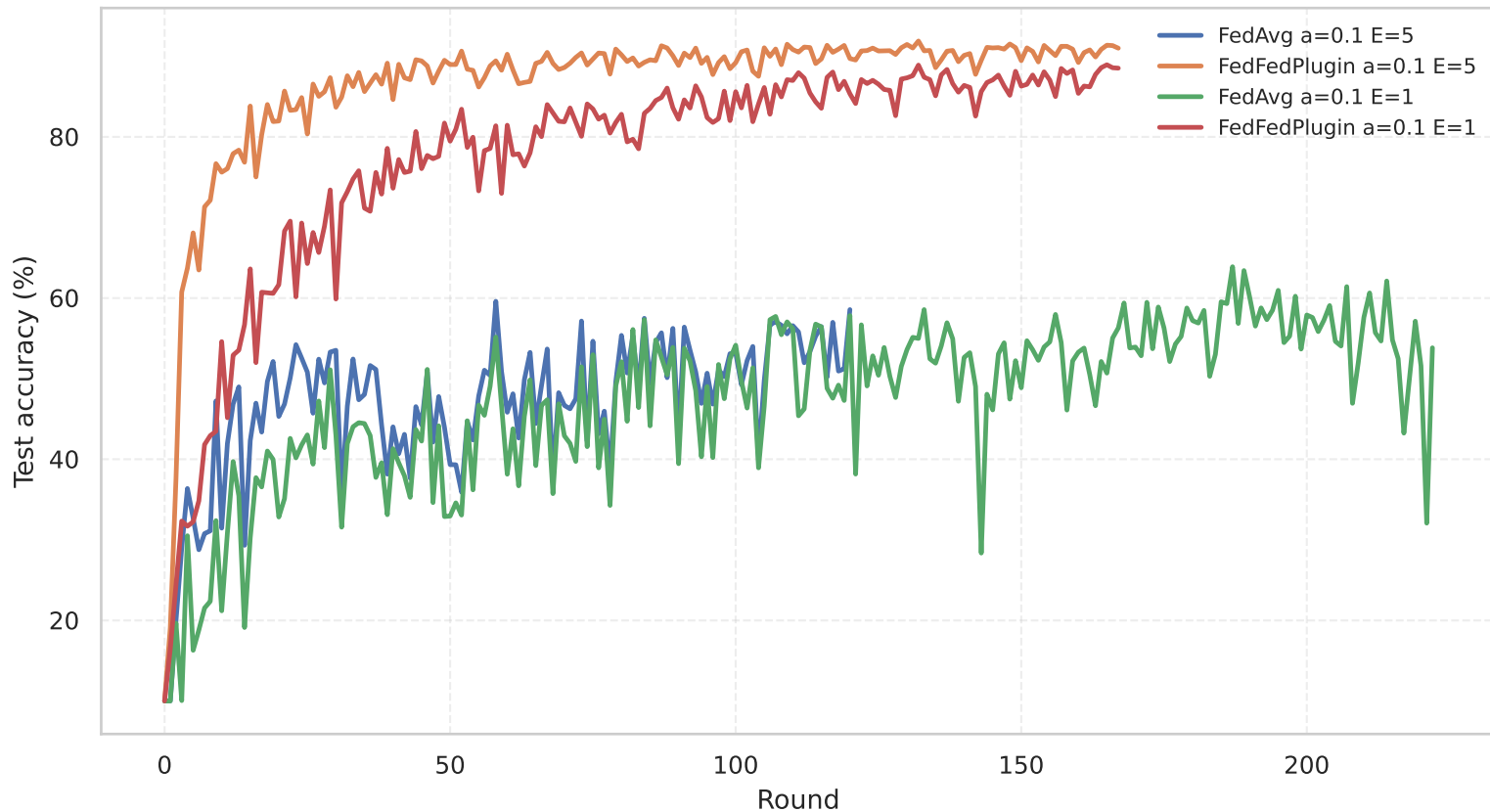
local_epoch: accuracy curves
