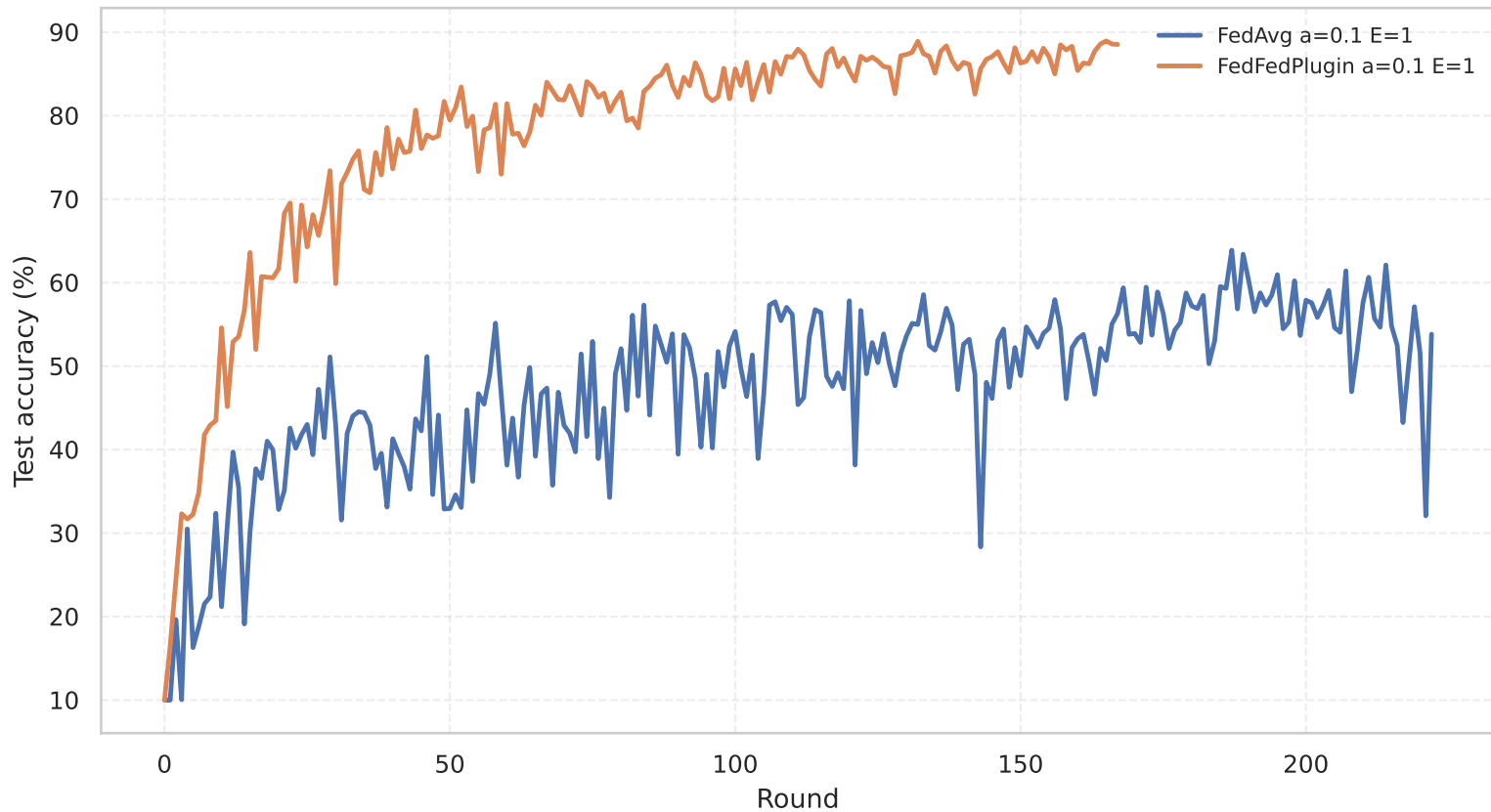
main_a0p1_e1: accuracy curves
